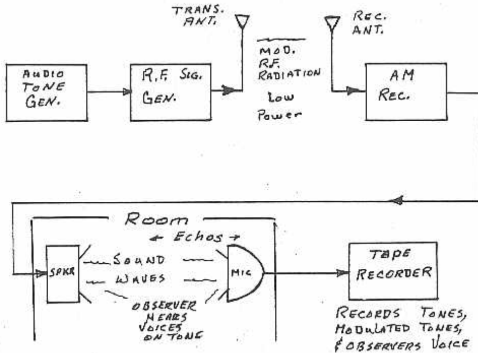
Fig. 11 Functional Block Diagram of Mark IV
